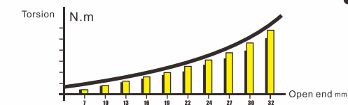
Open end and torsion diagram
